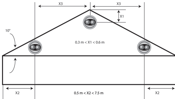
Pultdachmontage
